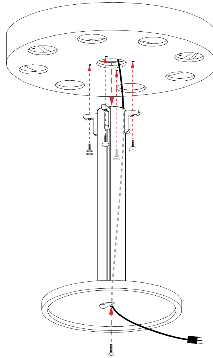
Underside View
